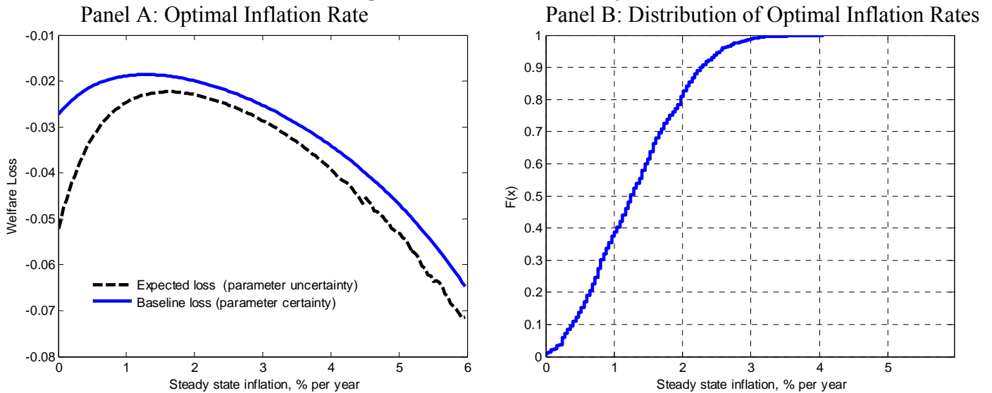
Figure 8. Model Uncertainty
